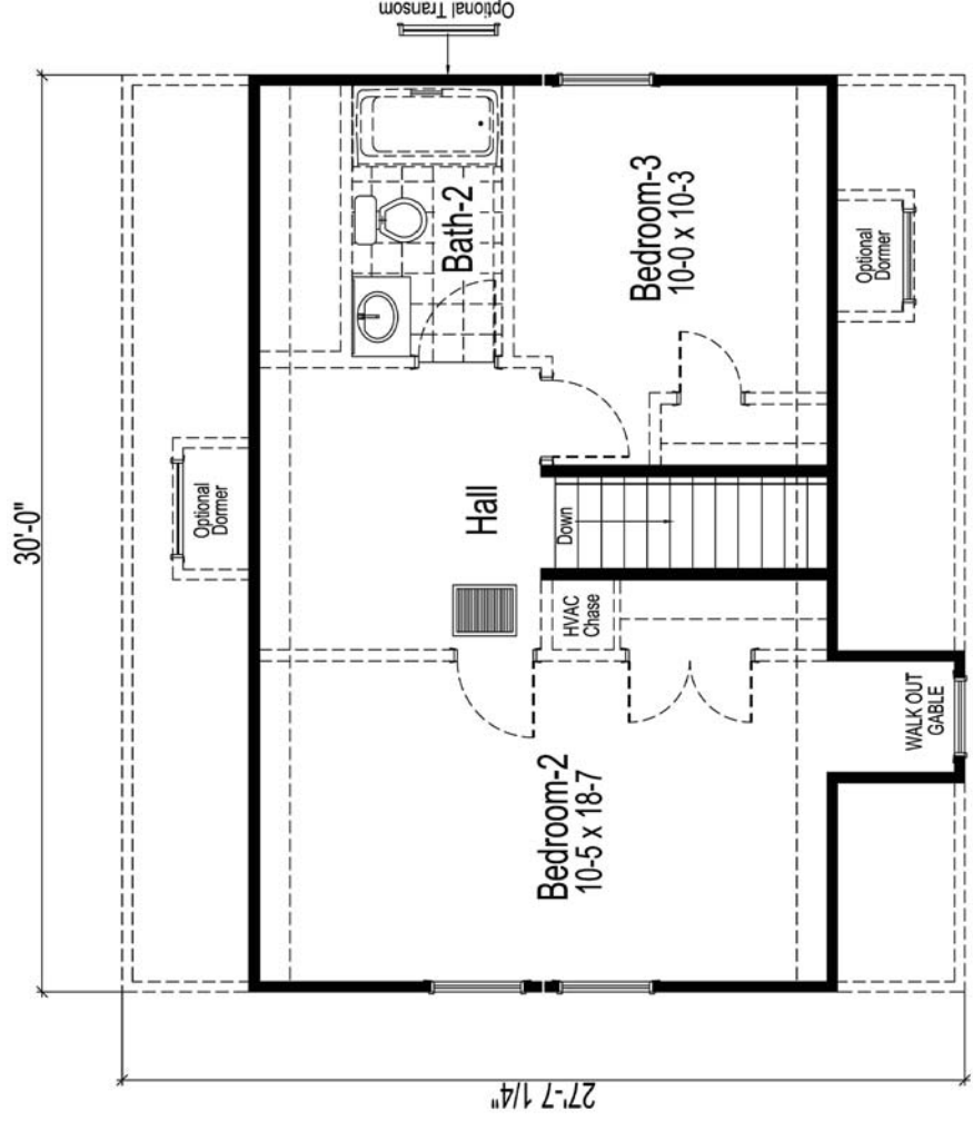
Opt. Basement Plan
